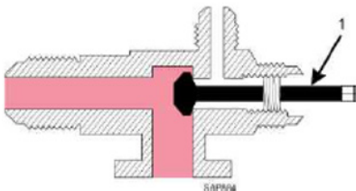
Service Valve Back Seated (Operating Position)
