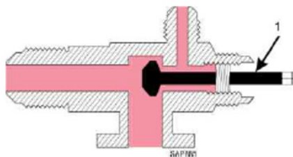
Service Valve Open to Port (Servicing Position)
