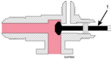
Service Valve Back Seated (Operating Position)
