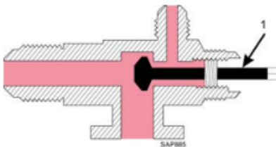
Service Valve Open to Port (Servicing Position)
