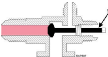
Service Valve Front Seated (Check or Remove Compressor)
